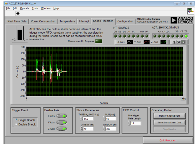
Figure 23. Shock Recorder Tab
