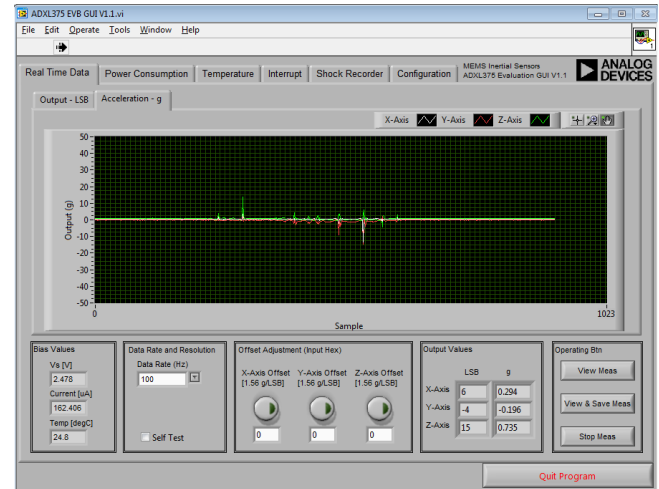
Figure 17. Real Time Data Tab
