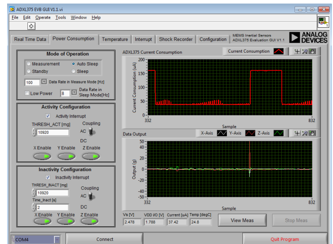
Figure 19. Auto Sleep Operation
