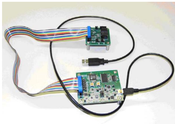
Figure 1. EVAL-ADXL375Z-M Evaluation System
