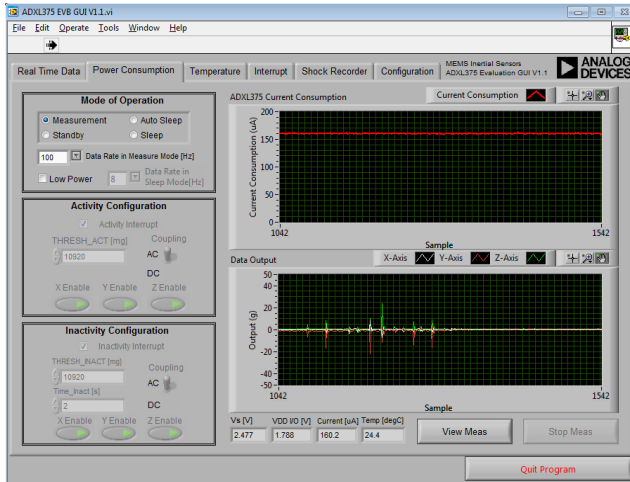
Figure 18. Power Consumption Tab
