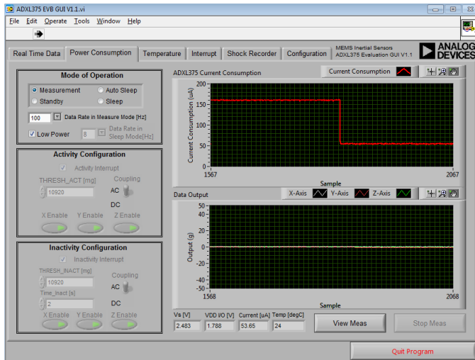
Figure 20. Low Power Operation
